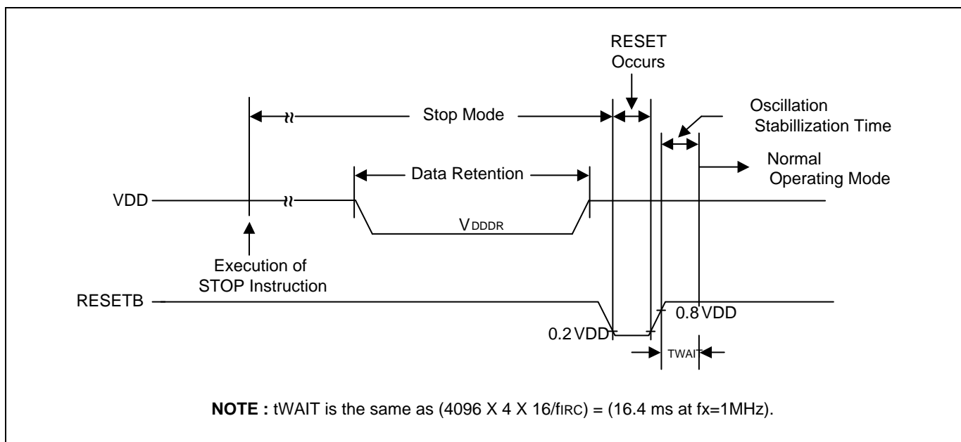
Figure 7.6 Stop Mode Release Timing when Initiated by RESETB
