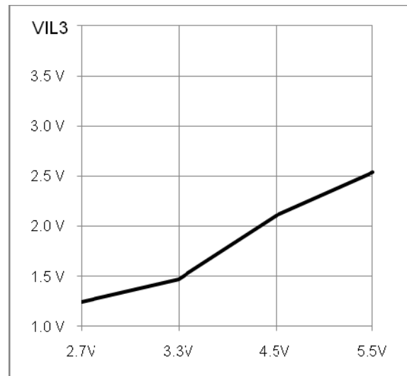
Figure 7-26 V_{IL3} - V_{DD}
