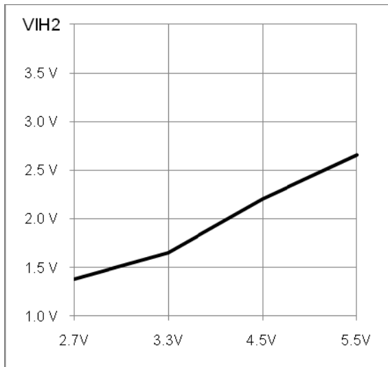
Figure 7-23 V_{IH2} - V_{DD}
