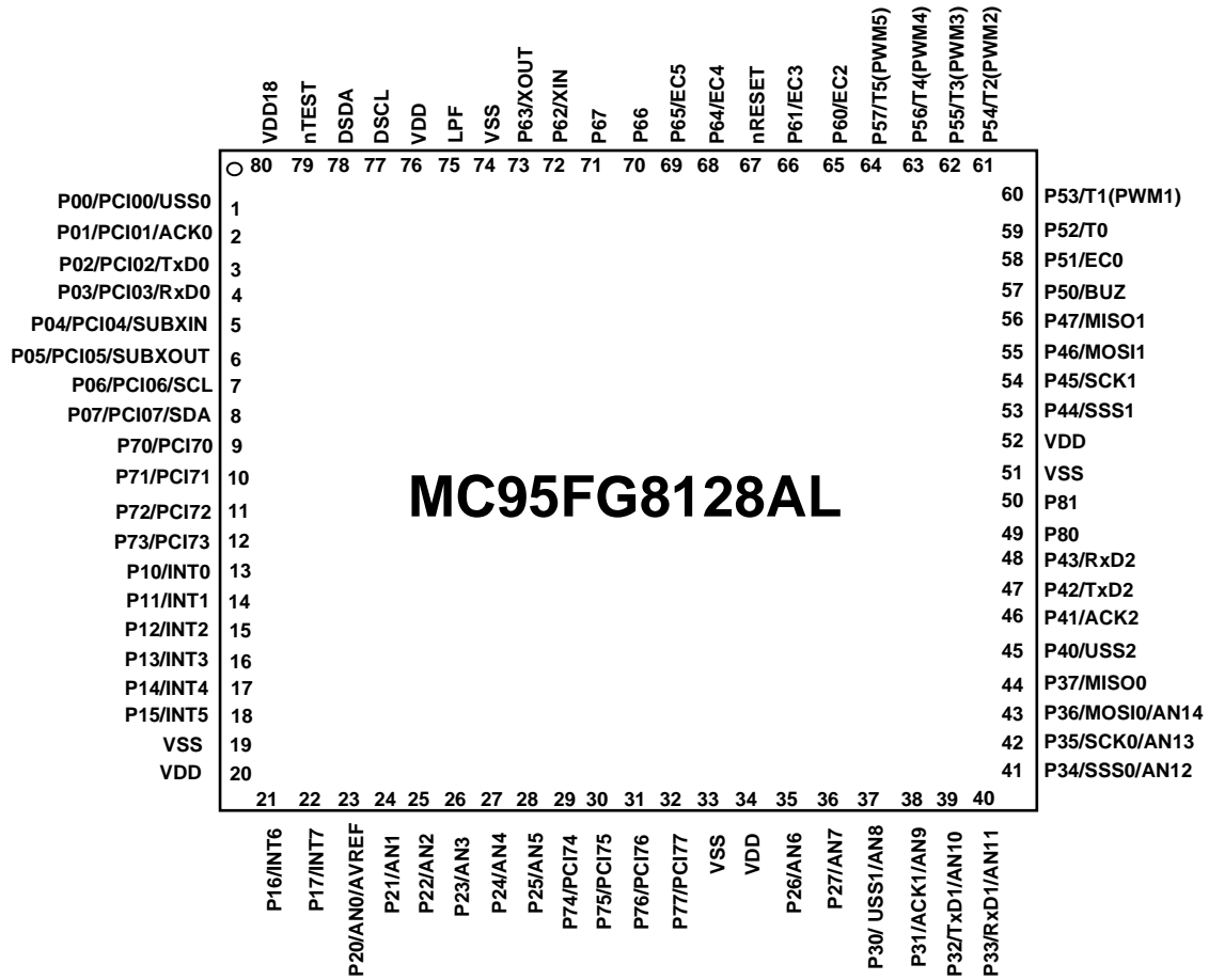
Figure 3.2 MC95FG0128A 80 Pin LQFP assignment
