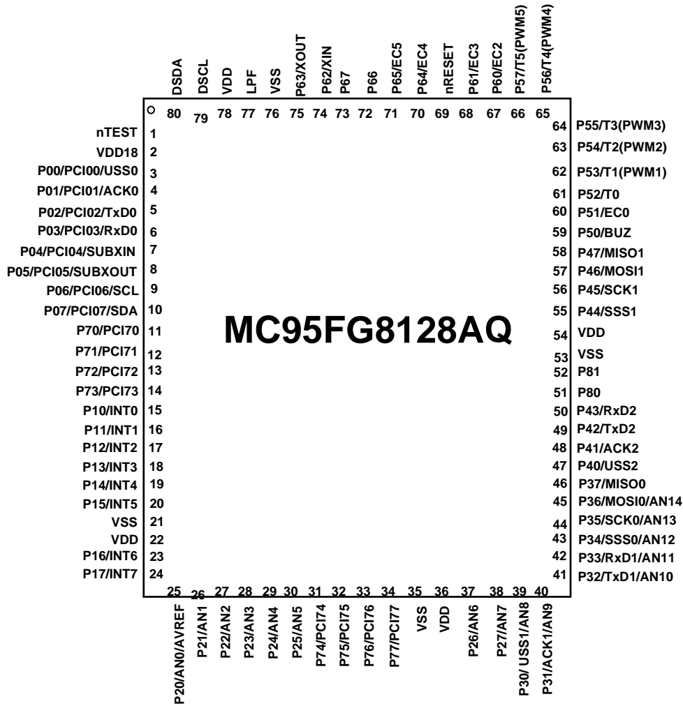
Figure 3-3 MC95FG0128A 80 Pin MQFP assignment
