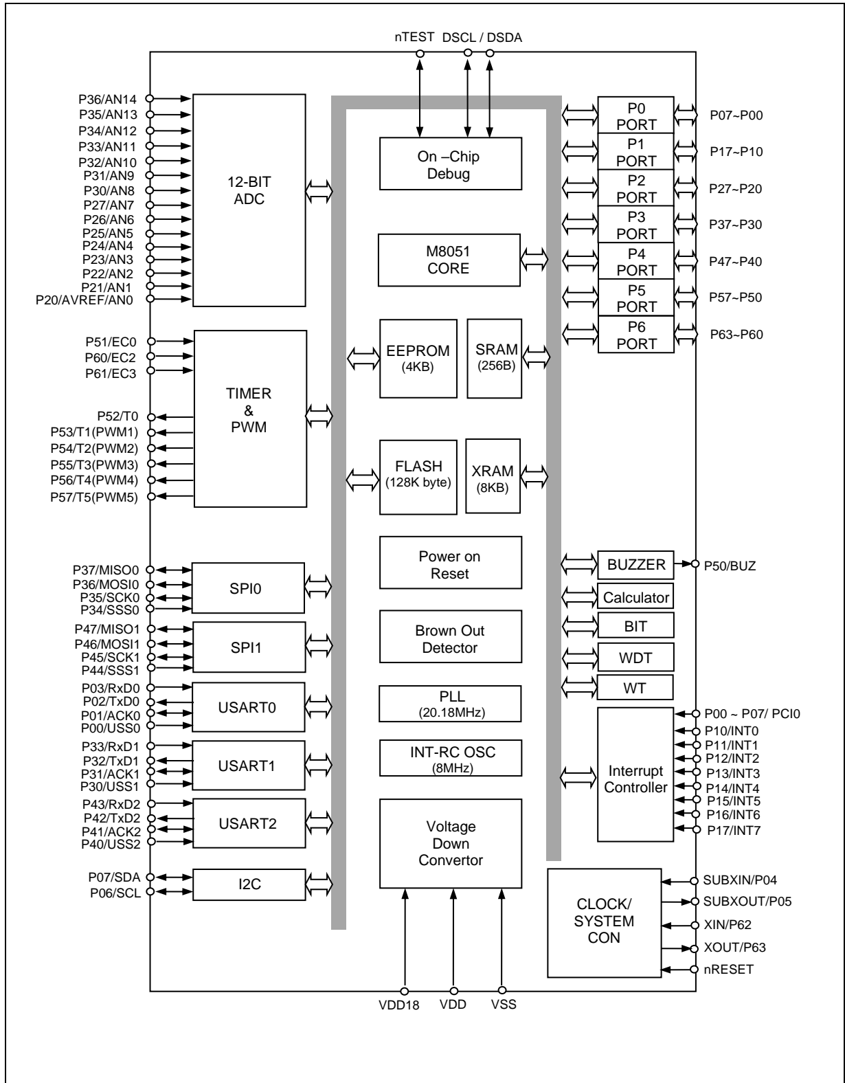
Figure 2.3 MC95FG6128A block diagram
