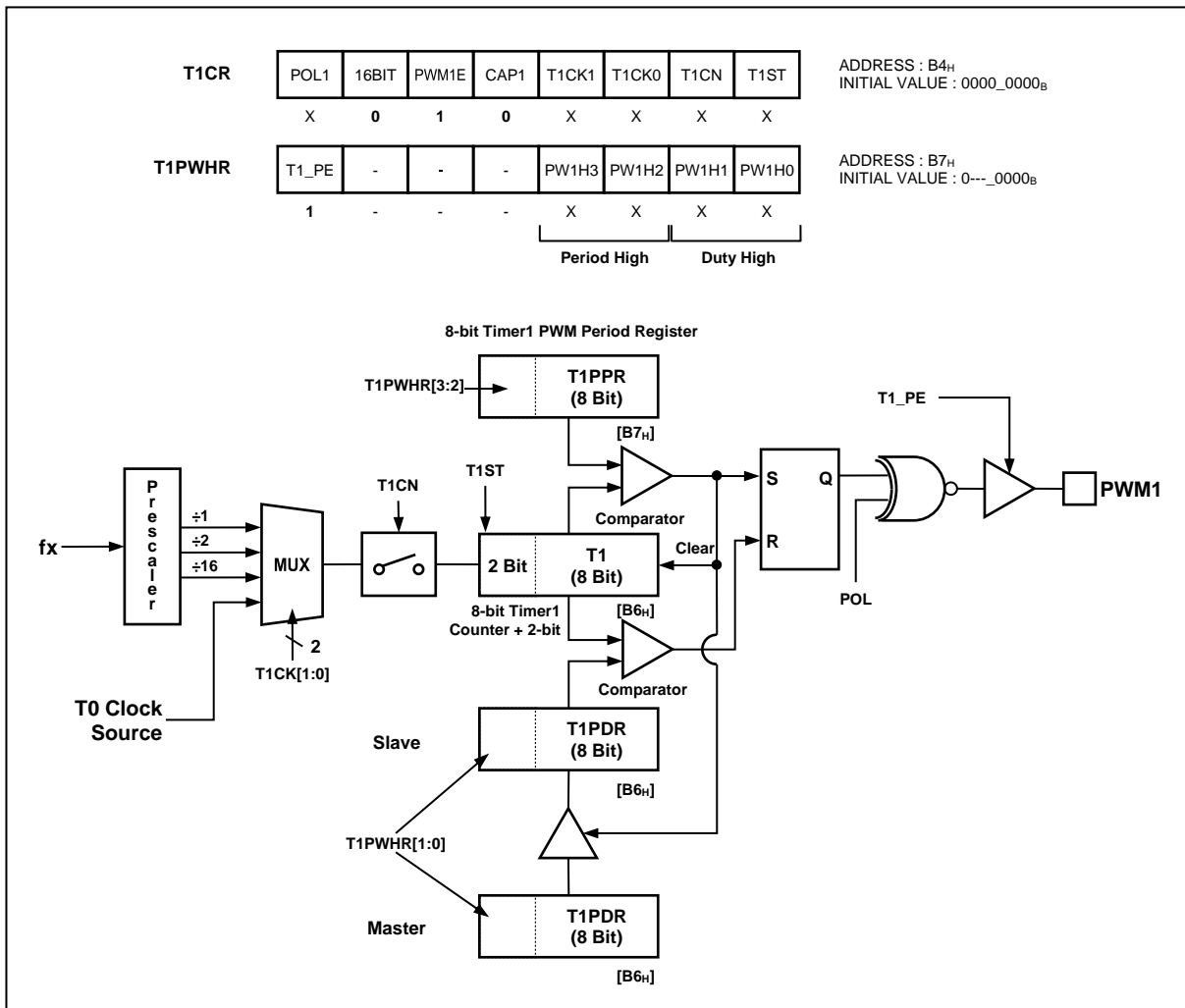
Figure 11.14 PWM Mode
