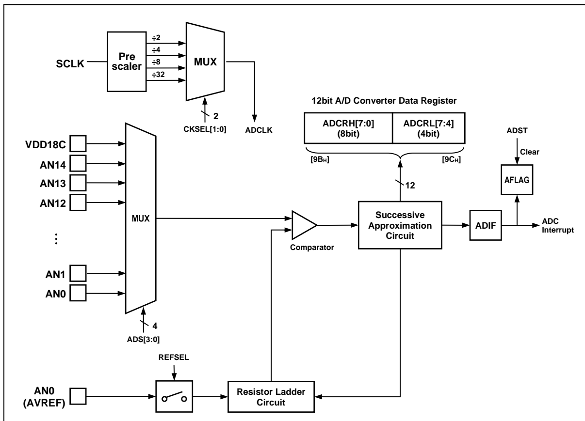
Figure 11.45 ADC Block Diagram
