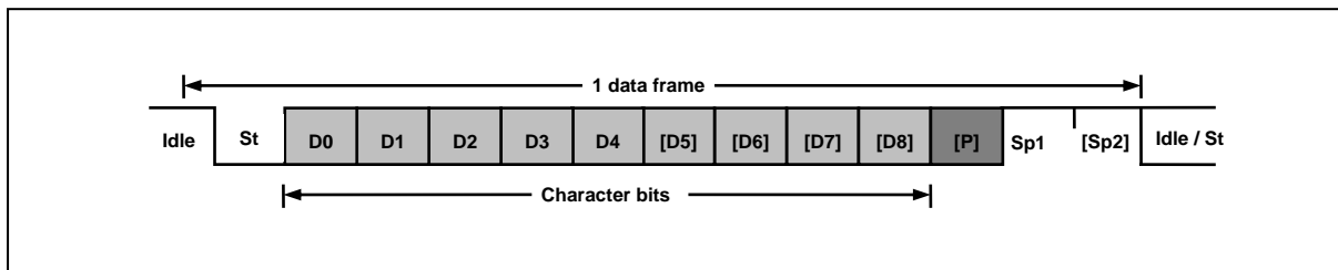
Figure 11.25 frame format
