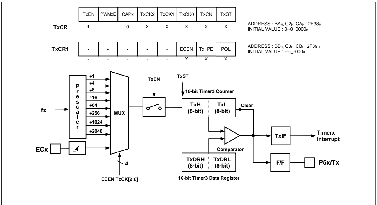
Figure 11.17 Timerx 16-bit Mode Block Diagram
