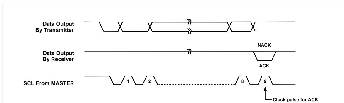
Figure 11.38 Acknowledge on the I 2 C-Bus
