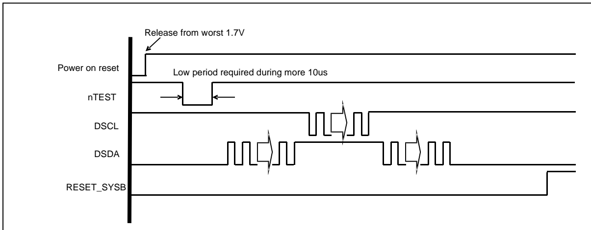
Figure 15.10 ISP mode
