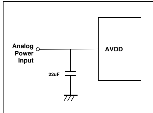
Figure 11.47 A/D Power(AVDD) Pin Connecting Capacitor
