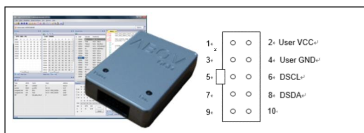
Figure 1.2 Debugger and Pin description
