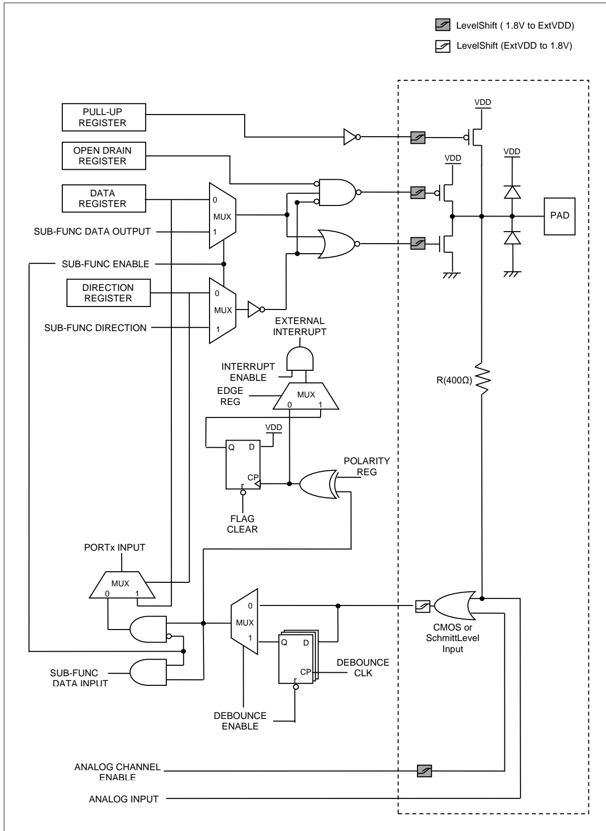
Figure 6.2 General Purpose I/O Port
