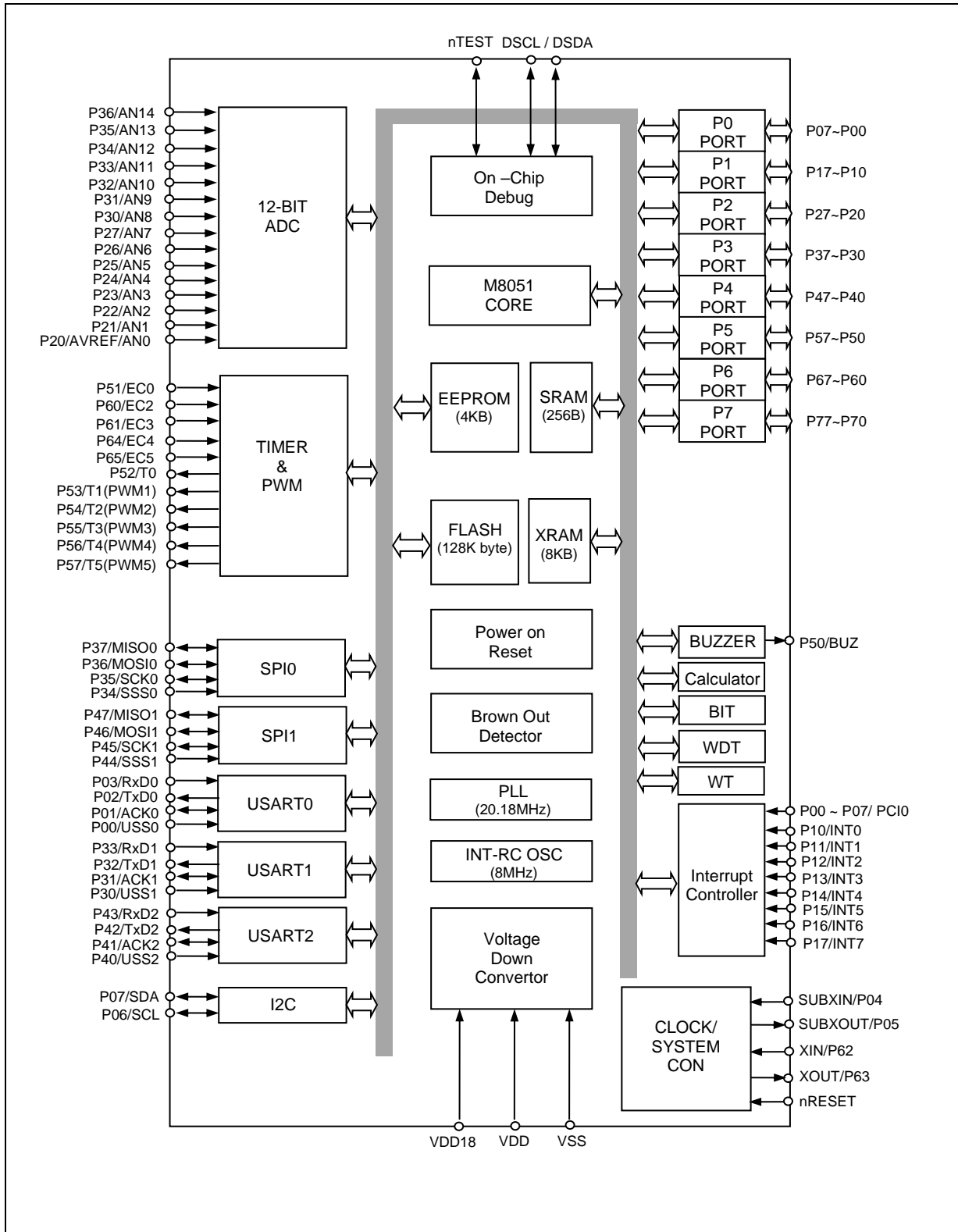
Figure 2.2 MC95FG8128A block diagram
