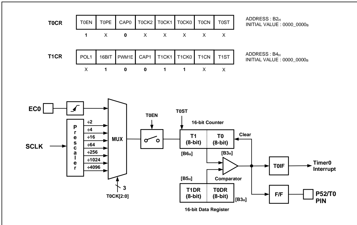
Figure 11.9 16 Bit Timer/Event Counter0, 1 Block Diagram
