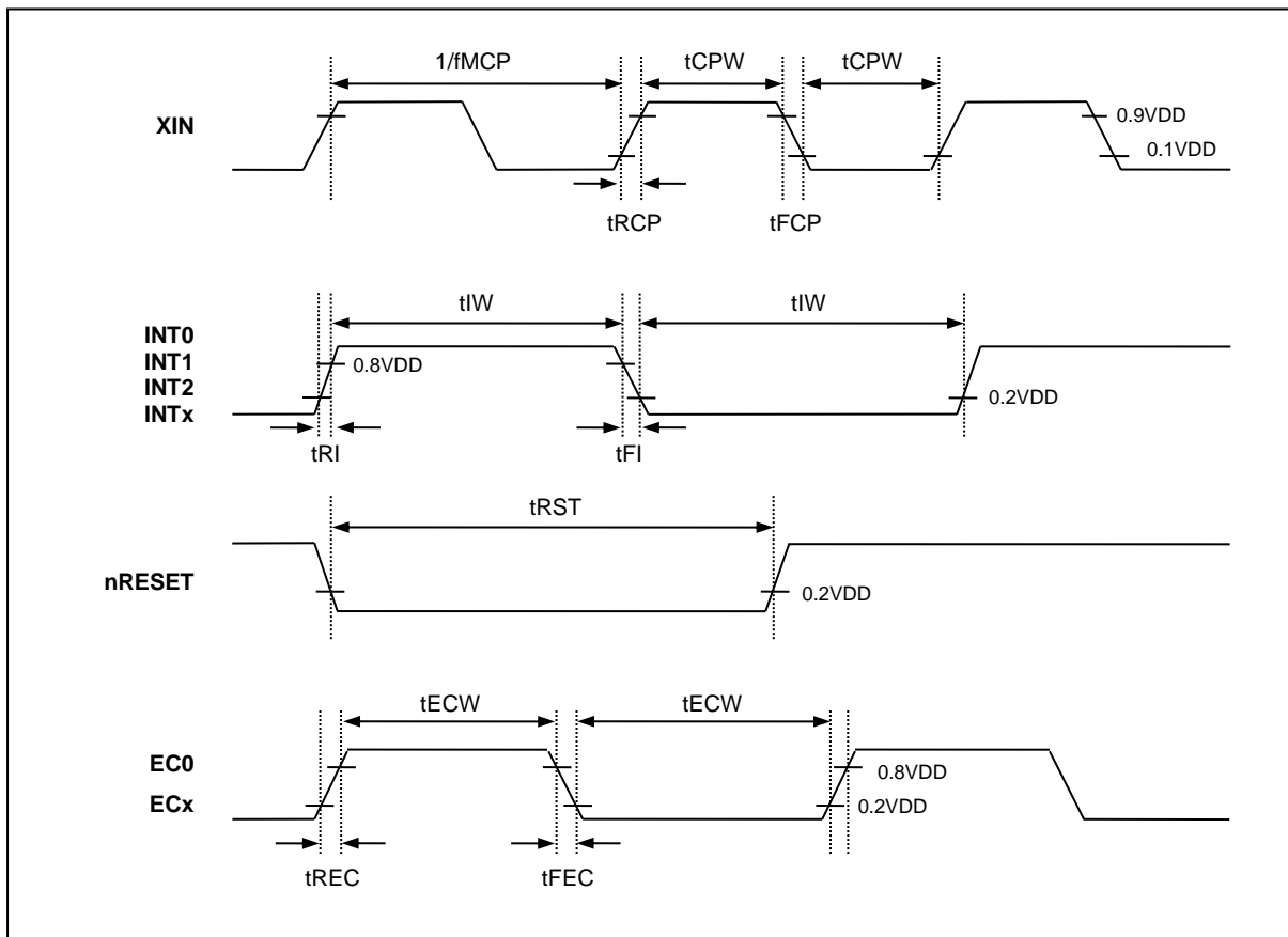
Figure 7.1 AC Timing
