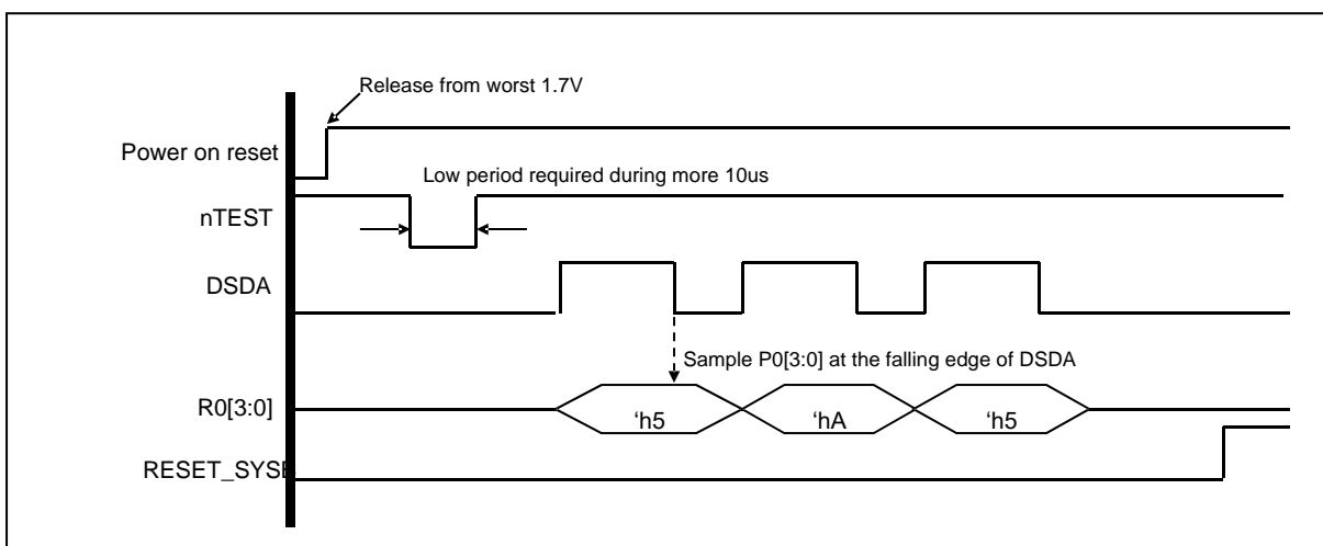
Figure 15.11 Byte-parallel mode
