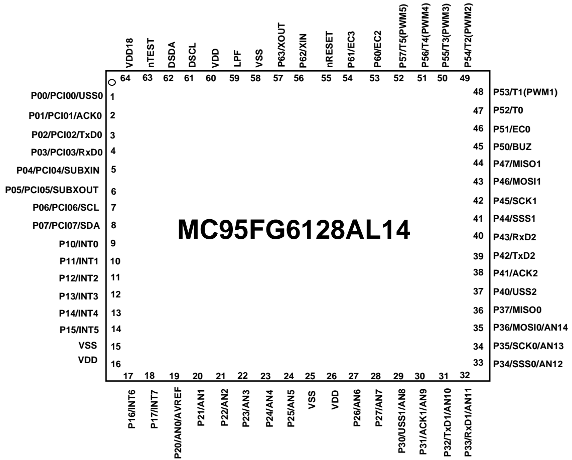
Figure 3-5 MC95FG0128A 64 pin LQFP14 assignment
