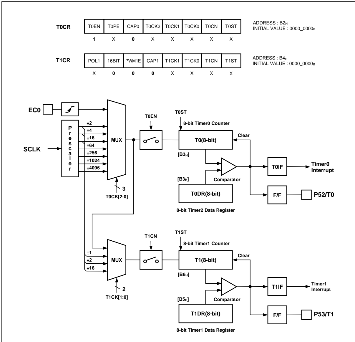
Figure 11.6 8 Bit Timer/Event Counter2, 3 Block Diagram
