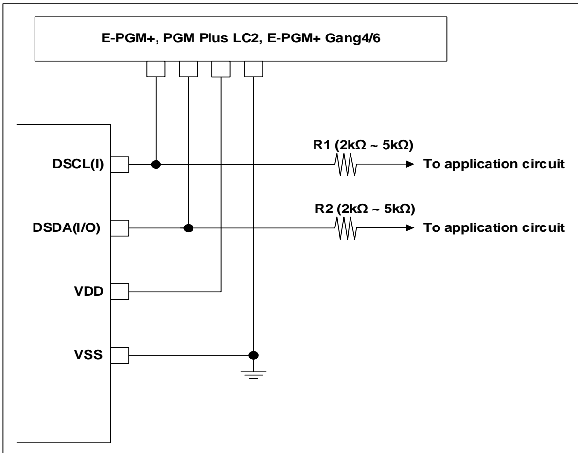
Figure 1.3 OCD Interface Circuit
