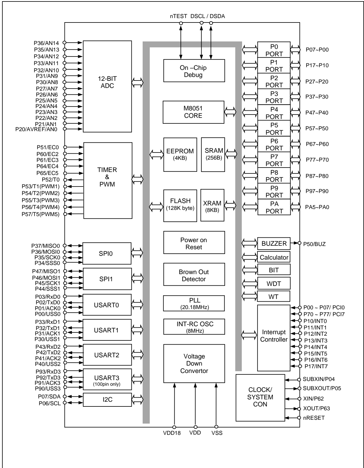
Figure 2.1 MC95FG0128A block diagram
